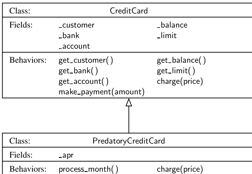
Figure 2.6: Diagram of an inheritance relationship.
