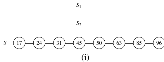
Figure 12.7: Example of an execution of the merge algorithm, as implemented in Code Fragment 12.3 using queues.
