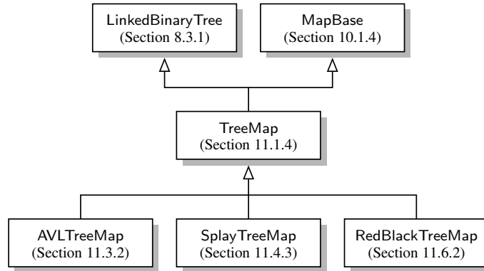
Figure 11.10: Our hierarchy of balanced search trees (with references to where they are defined). Recall that TreeMap inherits multiply from LinkedBinaryTree and MapBase .
